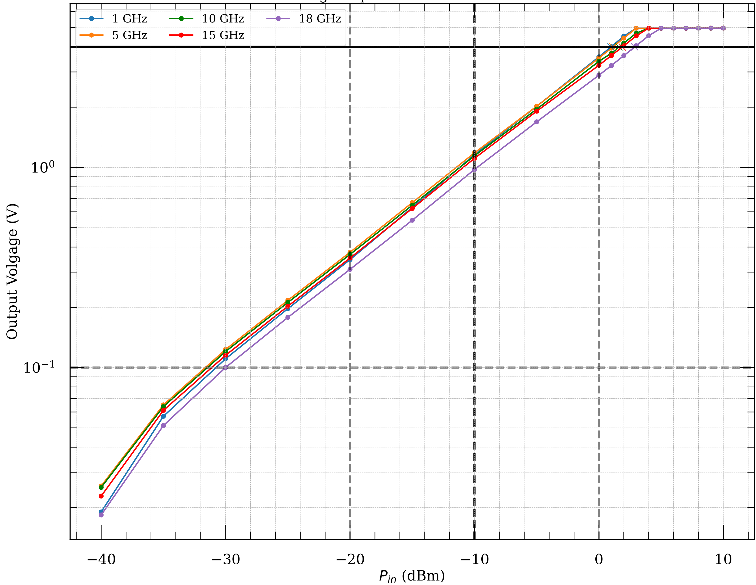
Measured voltage-to-power curve of detector module017
